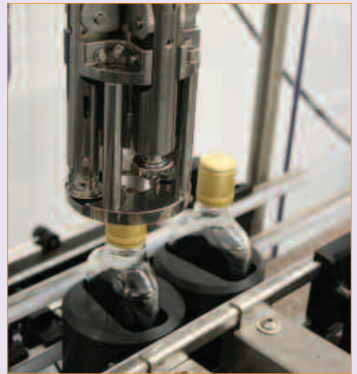
ROPP capping head
